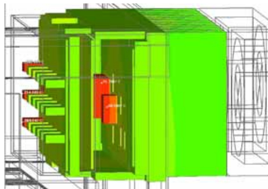
Datron needed fast and accurate simulation technology for natural convection studies to design a field radio.
