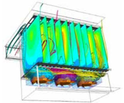
Velocity streamlines and temperature contours for card array in VME-format box cooled by three axial fans modeled using moving reference frame (MRF) fan model. The ANSYS Fluent solver enables fans to be modeled with actual fan geometry and rotational speed.
