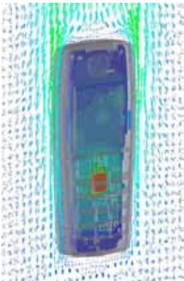
Velocity vectors and internal temperatures for cell phone assembly cooled by free convection
