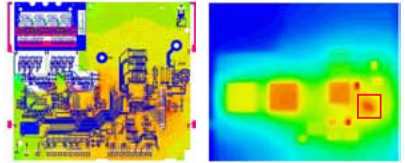
Coupling ANSYS Icepak with ANSYS SIwave (left) provides additional insight into local hotspots (right) from copper resistive losses in PCBs and packages.
