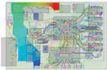
Electric potential contours on PCB trace; Joule heating of high current trace calculated as part of conjugate heat transfer solution
