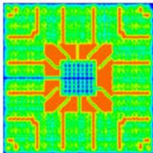
Detailed thermal conductivity map for IC package substrate layer computed based on electronic trace and via information
