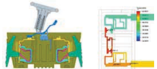
Schneider Electric used Icepak for thermal and electrical simulations on a wiring system switch device assembly to determine temperature and define conductor and insulator specifications.
