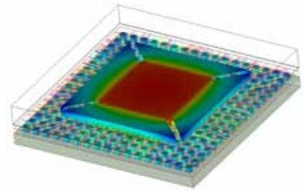
Temperature contours on a 272-pin ball grid array package on a substrate, package data imported from MCM file
