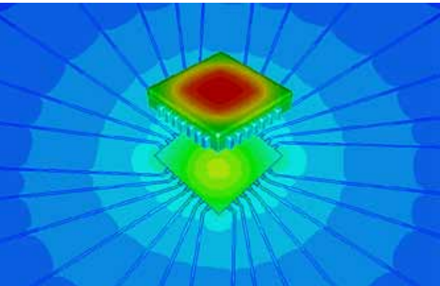
Temperature contours on micro lead-frame plastic quad (MLPQ) package in natural convection chamber
