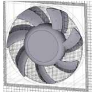
Multi-level hex-dominant mesh of fan represented directly as 3-D CAD geometry. Hanging-node mesh accurately resolves curved fan blade geometry.
