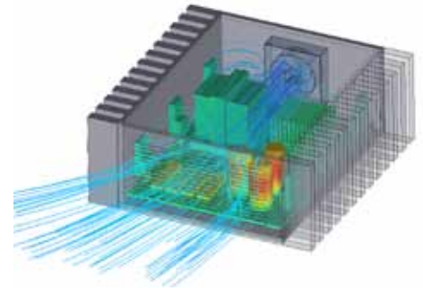
Velocity streamlines and temperature contours for fan-cooled avionics box exposed to solar radiation; model combines MCAD data and Icepak objects
