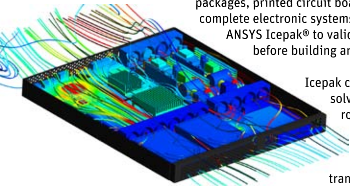
Fluid streamlines and temperature contours for 1U network server. Multi-level hex-dominant mesh accurately represents the complex geometry.
