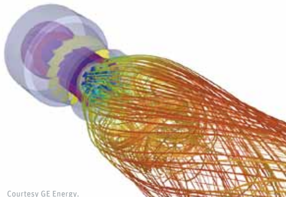
Fluent’s advanced reacting flow models tackle a vast array of gaseous, coal and liquid fuel combustion simulations, such as this low NOx burner.
